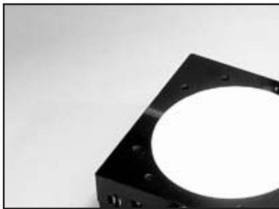
Optional X-Y stage provides 30 x 30mm of movement to 1 \mu M resolution
